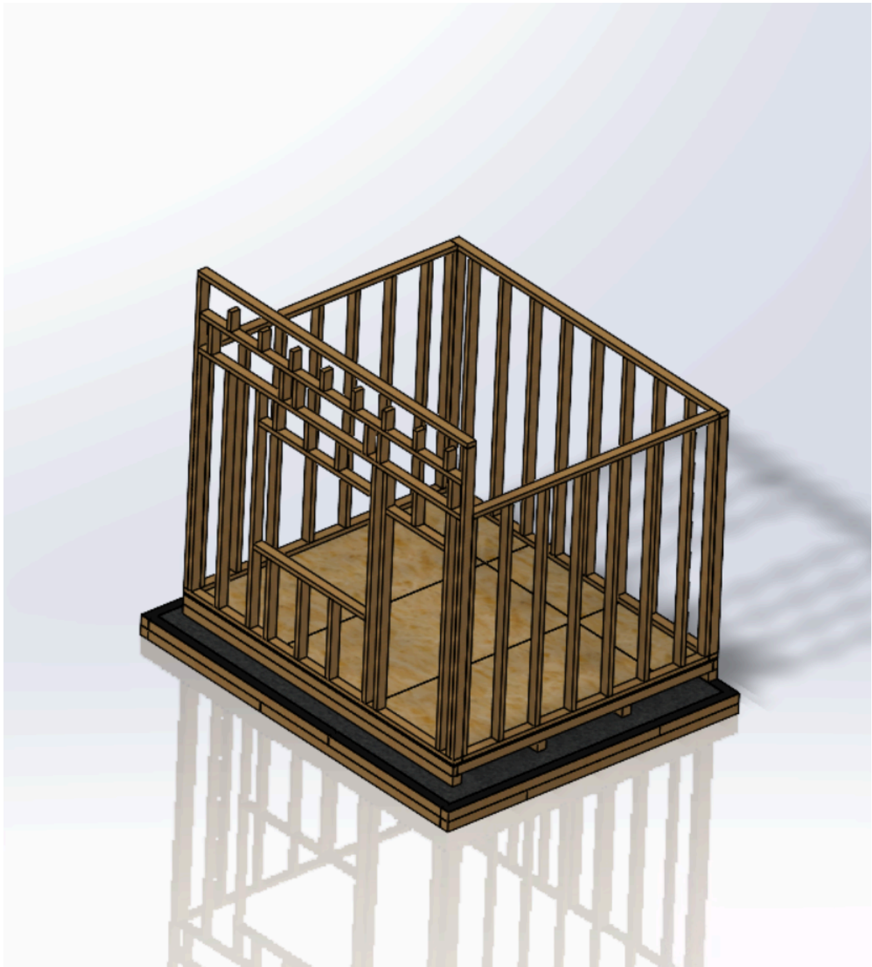
Figure 1.11: Original CAD concept of shed
